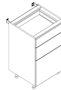
Bas 1 casserolier + 1 gd tiroir + 1 tiroir L.400/600/800/1000
